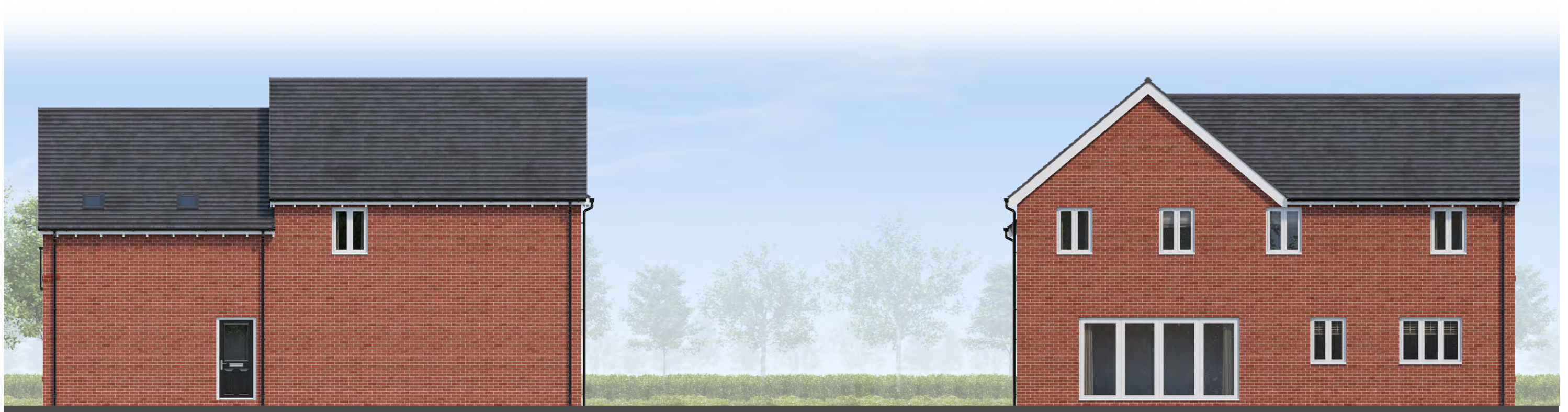
Rear Elevation
