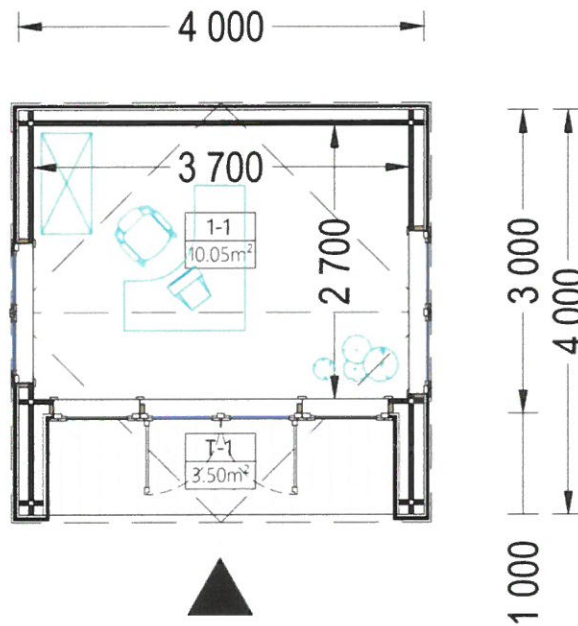
Floor plan Scale 1:750
