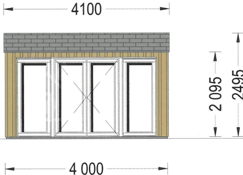
Front Elevation Scale 1:570
