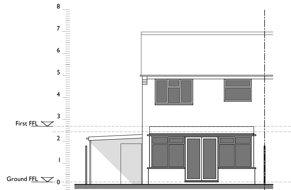
Existing - South Elevation 1:100
