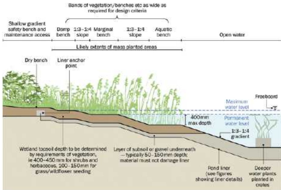
Figure 23.5 Typical planted pond edge details
