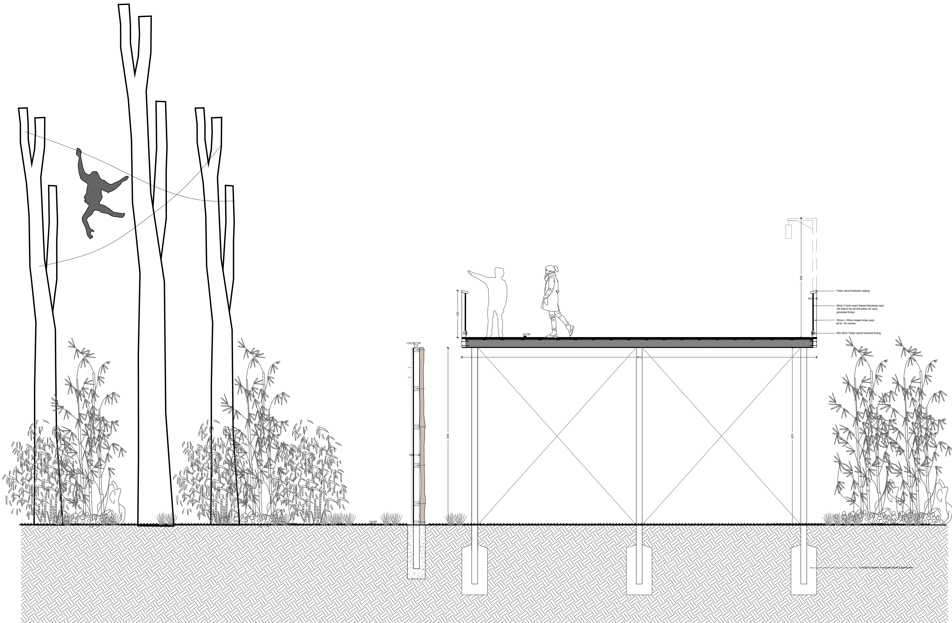
CROSS SECTION - through high level boardwalk at entrance to Orangutan House
