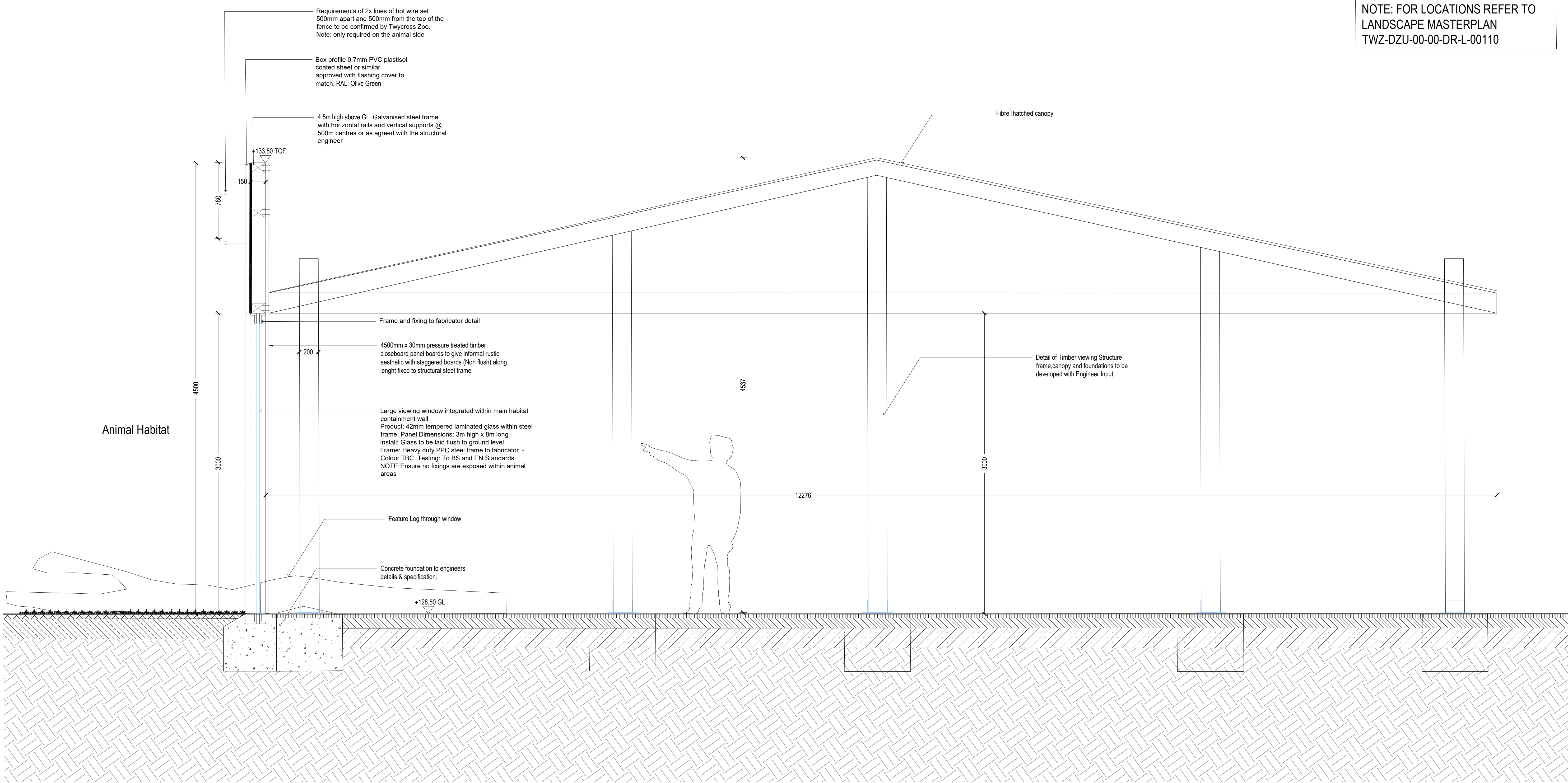
F3 4.5m High box profile sheet metal fence with integrated viewing window detail and viewing canopy Scale: 1:20
