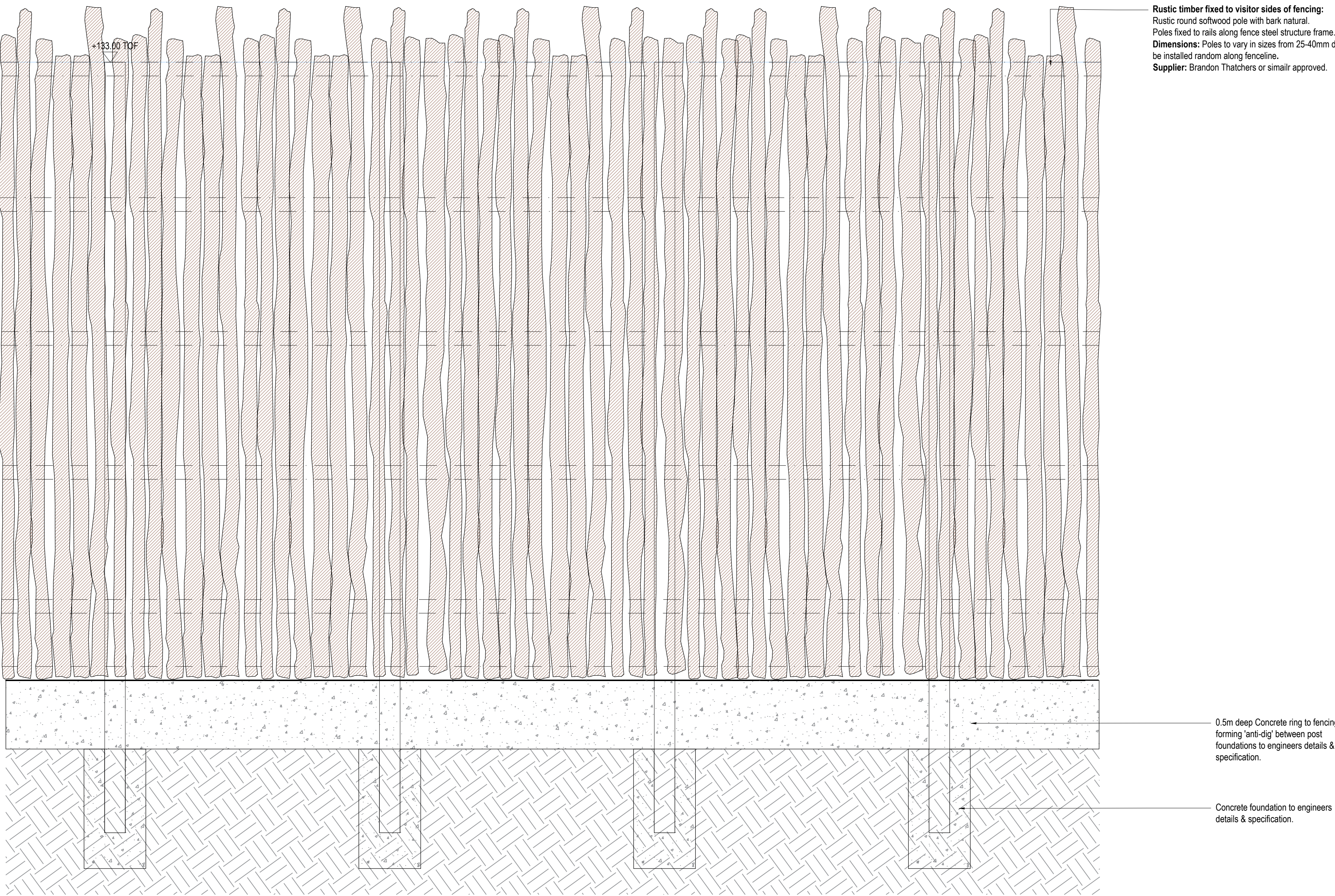
F2A 4.5m High visitor facing timber cladding elevation
