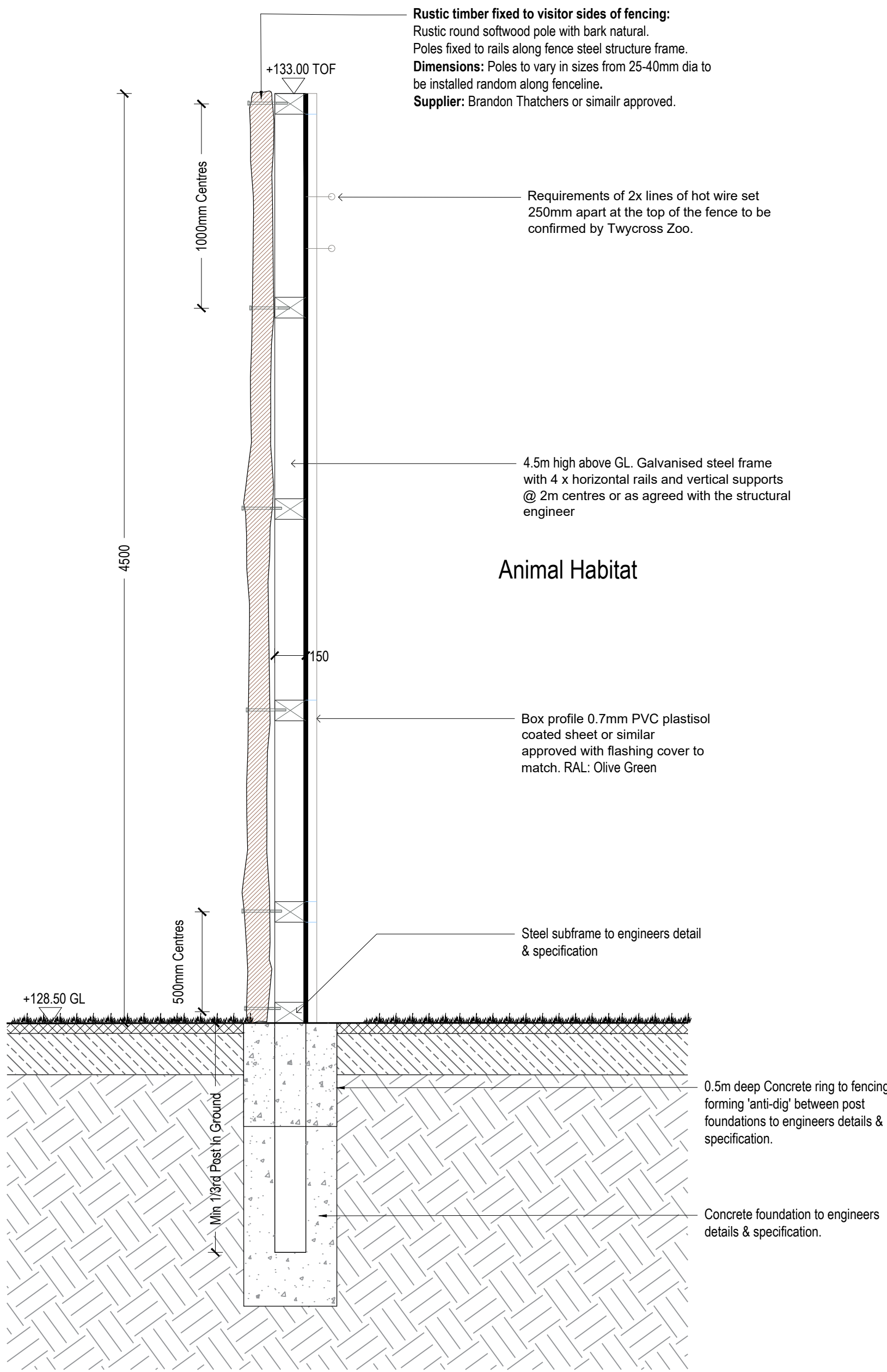
F2A 4.5m High box profile sheet metal fence with visitor facing Timber cladding detail
