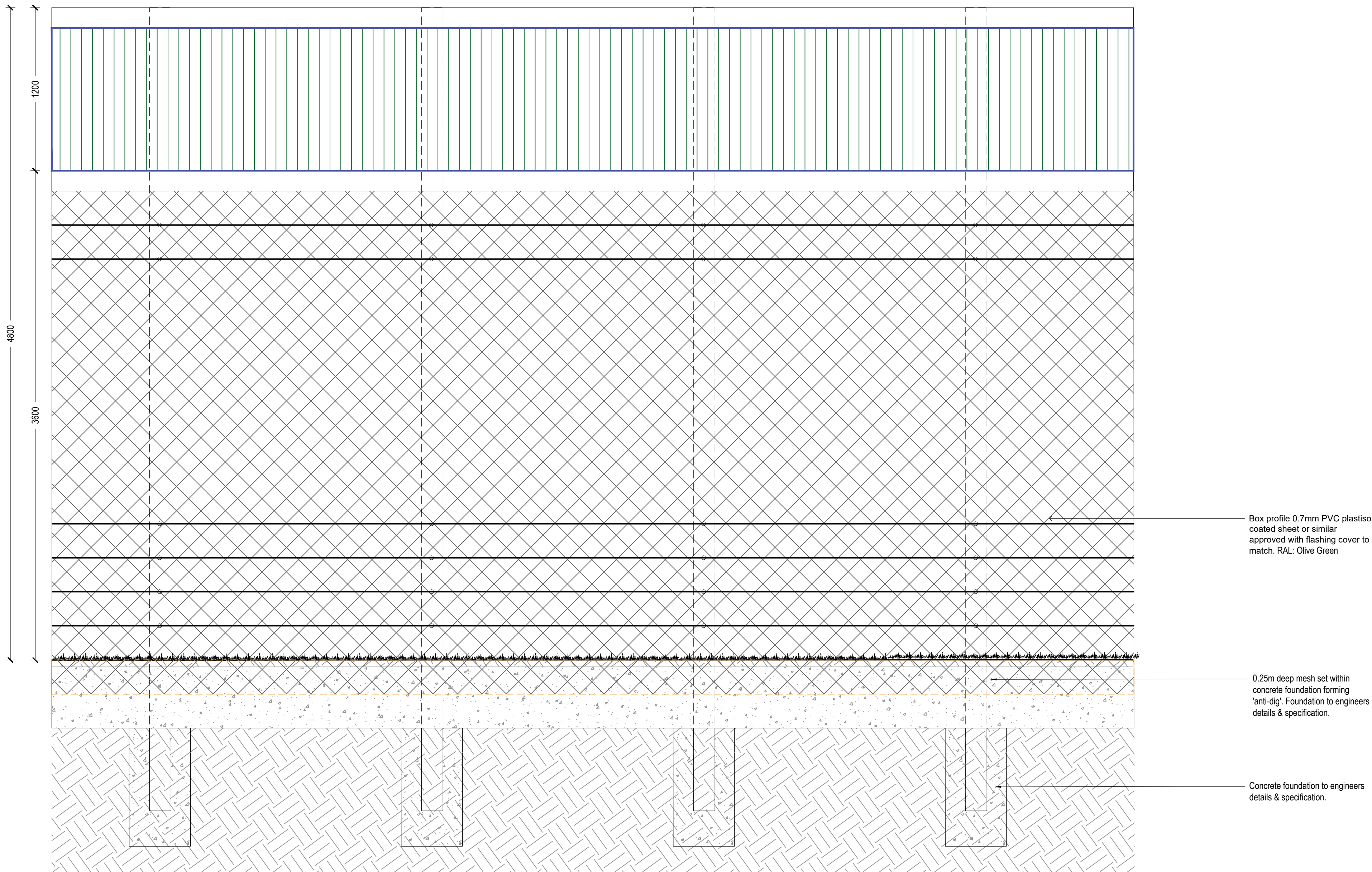
F1 4.5m High fence with Timber post, chainlink and anticlimb Elevation Scale: 1:20
