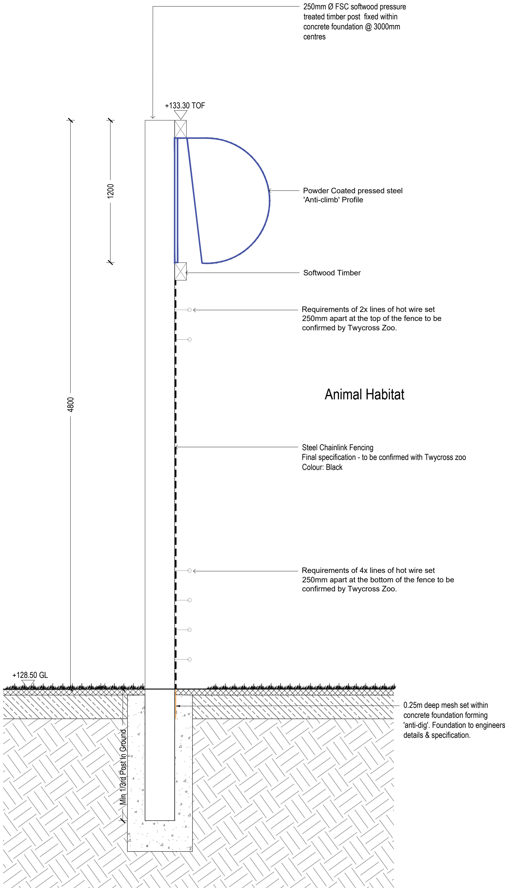
F1 4.5m High fence with Timber post, chainlink and anticlimb Scale: 1:20
