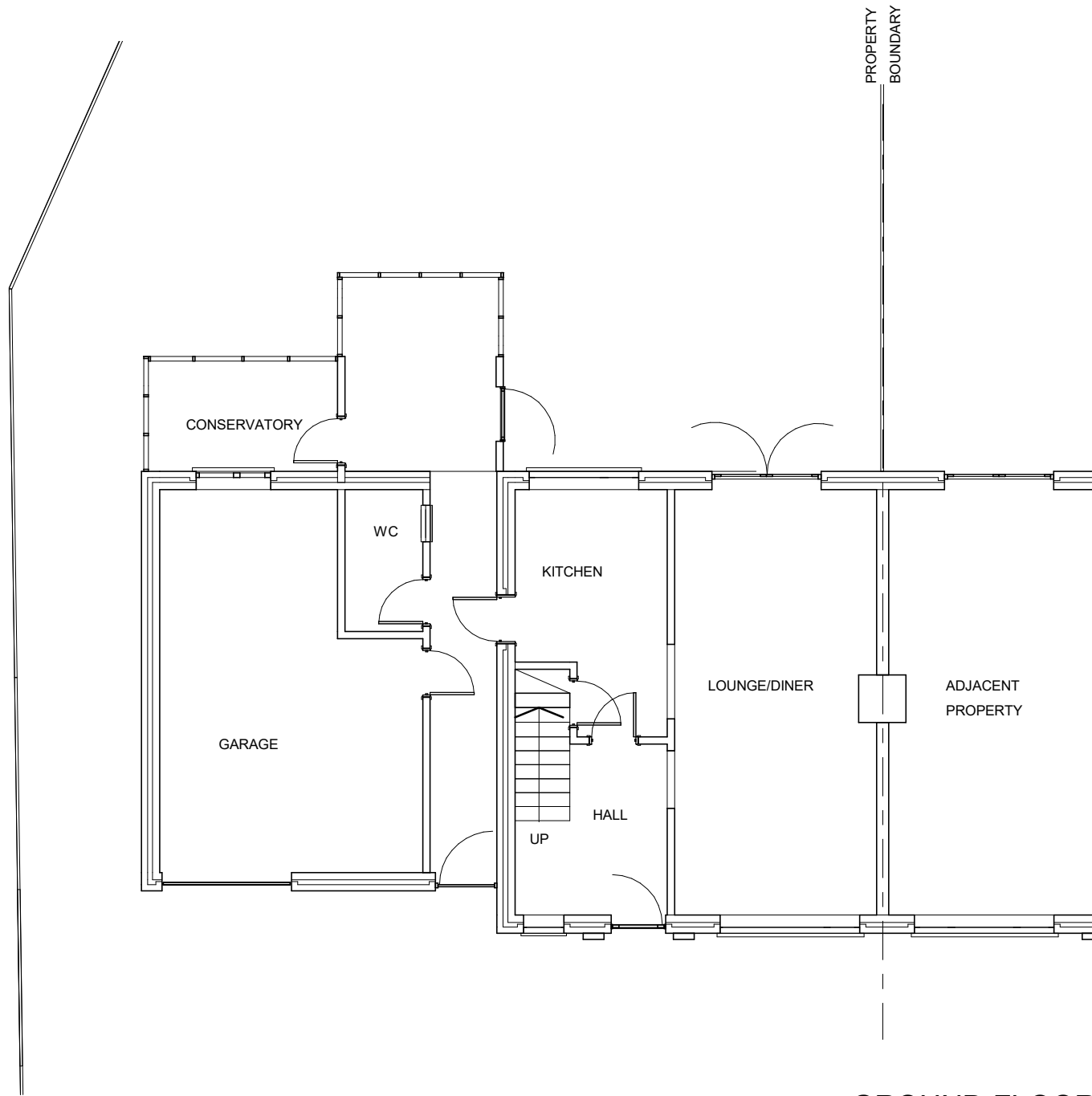
GROUND FLOOR
