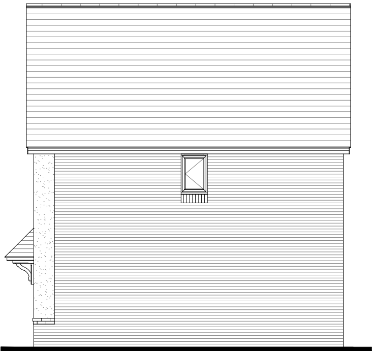
Side Elevation
