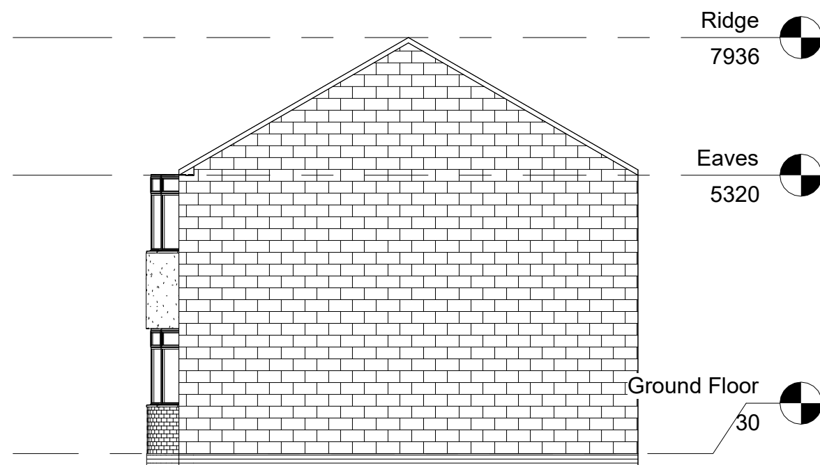
3 Proposed Side 1 Elevation 1 : 100
