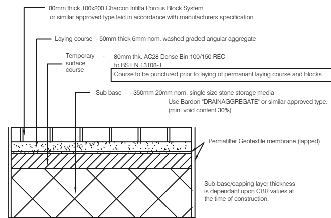
BLOCK PAVING SHARED DRIVE
