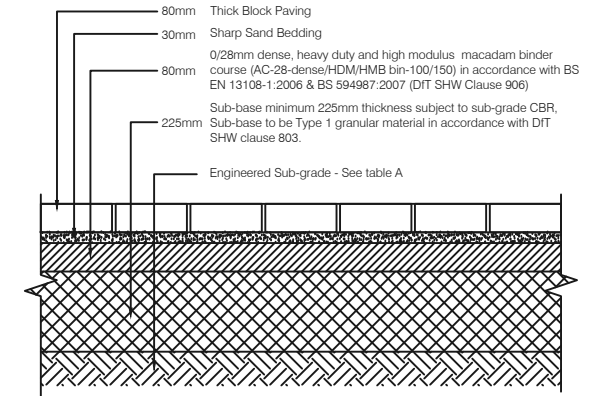
BLOCK PAVED AREAS ACCESSIBLE TO COMMERCIAL OR REFUSE VEHICLES
