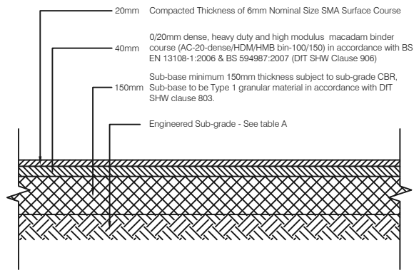
BITUMINOUS PRIVATE DRIVE
