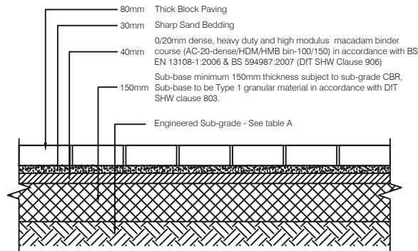
BLOCK PAVING PRIVATE DRIVE
