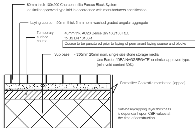
BLOCK PAVING PRIVATE DRIVE
