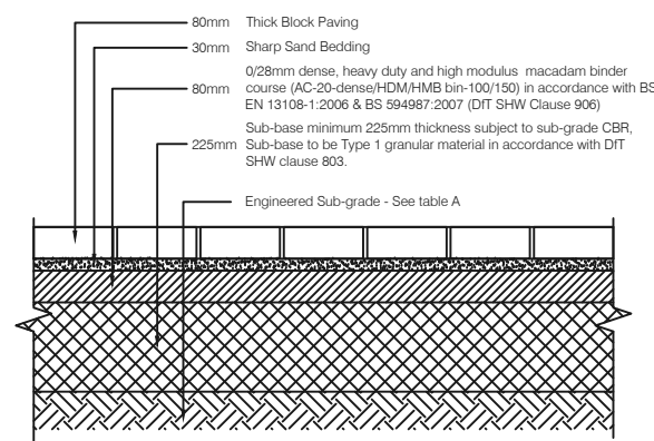
BLOCK PAVING SHARED DRIVE
