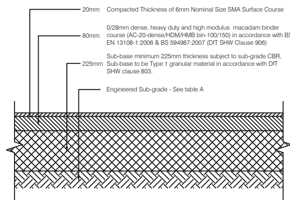
BITUMINOUS SHARED DRIVE
