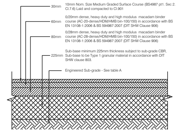
BITUMINOUS AREAS ACCESSIBLE TO COMMERCIAL OR REFUSE VEHICLES
