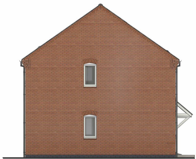
Left Elevation
