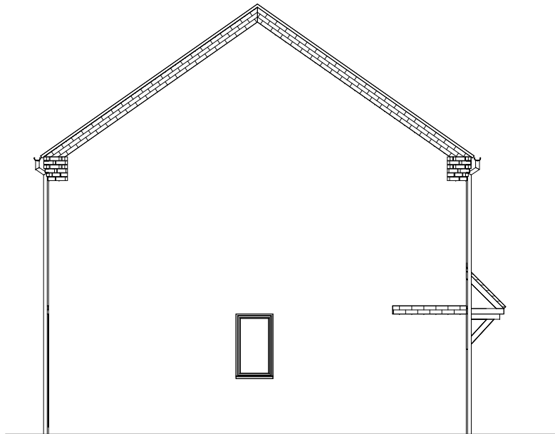
Left Elevation
