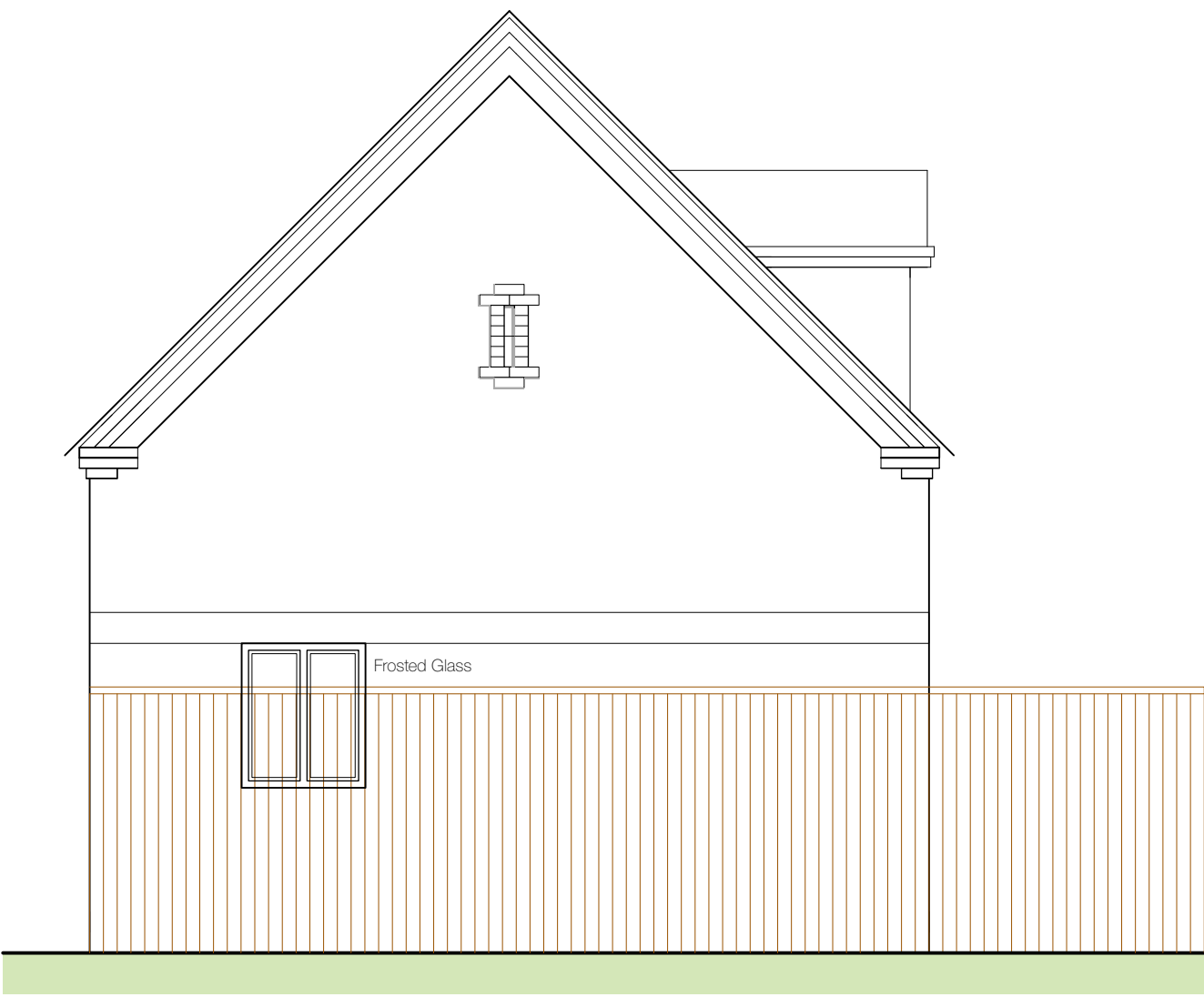
East Elevation
