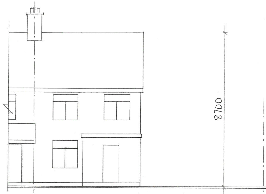
EXISTING REAR ELEVATION - N
