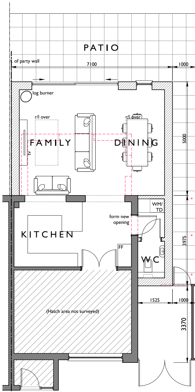
Proposed - Ground Floor Plan 1:100 0 1m 2m 3m 4m 5m NORTH
