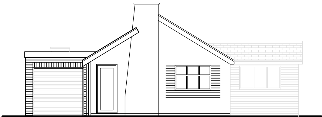
Front Elevation 1:100
