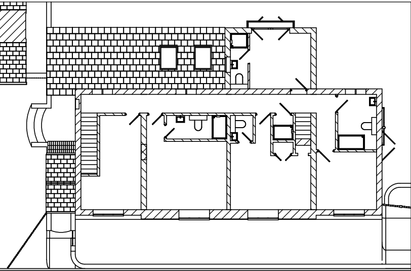
PROPOSED UPPER FLOOR - SECTION PLAN
