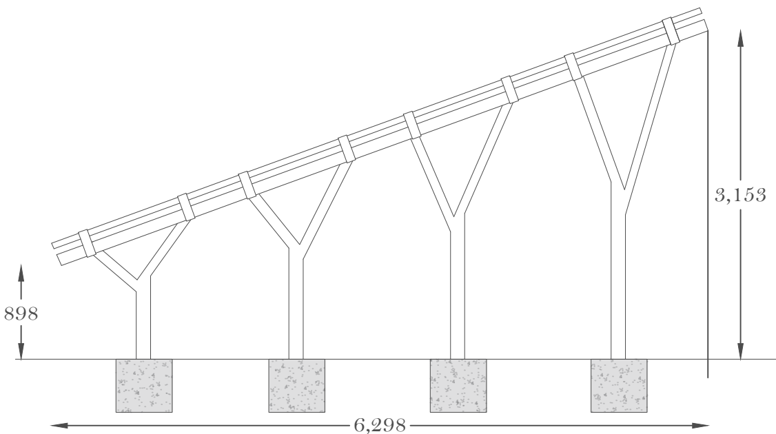
Proposed : Solar Panel Elevation 03 @ 1:50
