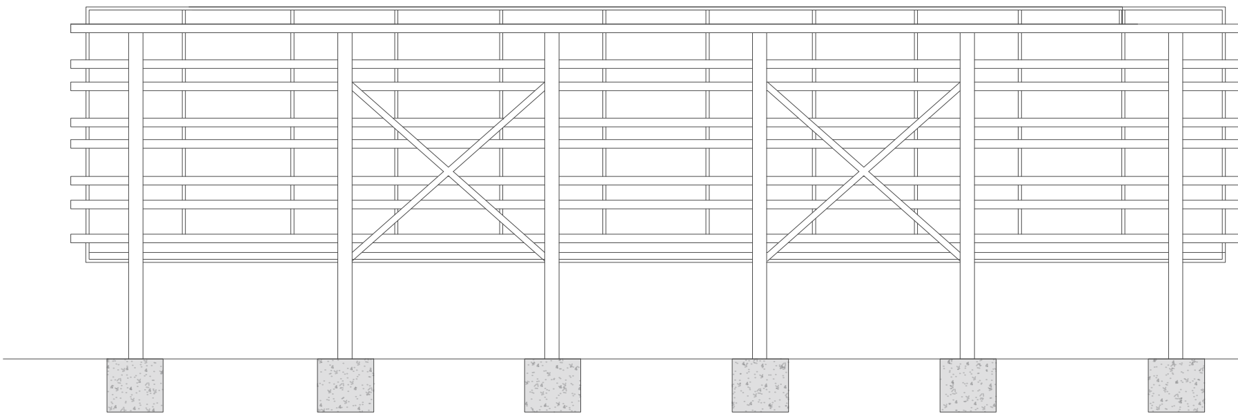
Proposed : Solar Panel Elevation 01 @ 1:50
