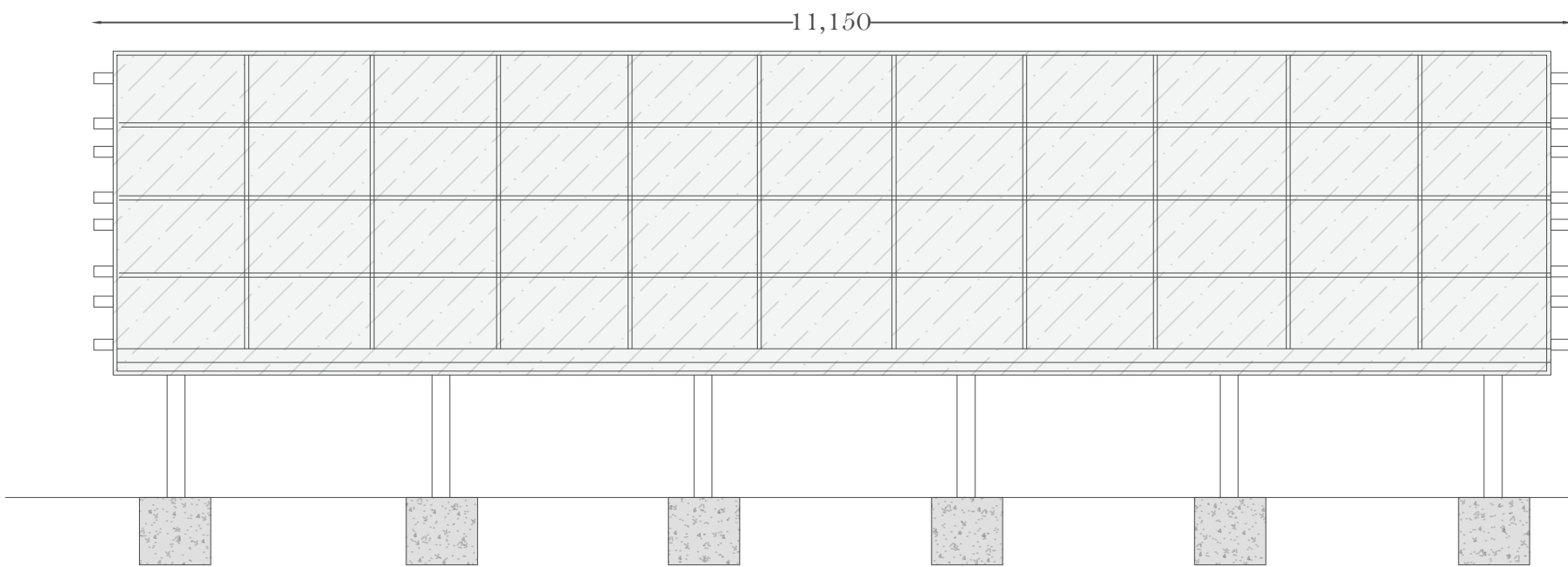
Proposed : Solar Panel Elevation 02 @ 1:50
