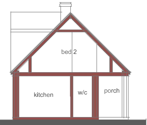
section through
