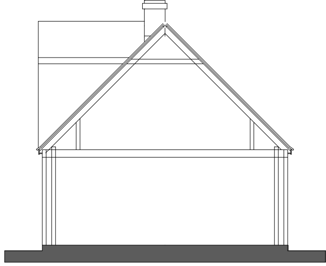
section through
