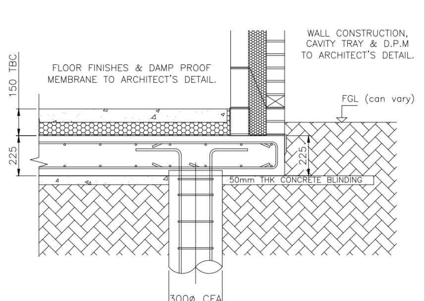
TYPICAL STRAIGHT SHUTTERED SLAB EDGE DETAIL WITHOUT HEAVE PRECAUTIONS
