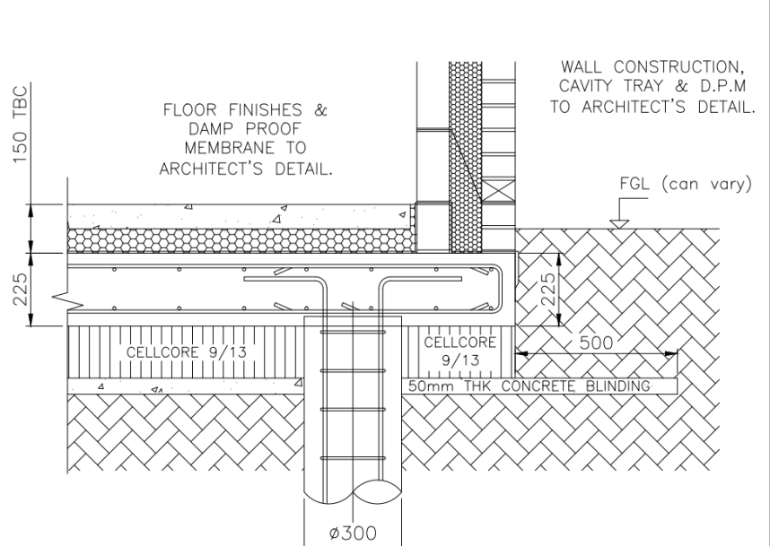
TYPICAL STRAIGHT SHUTTERED SLAB EDGE DETAIL WITH HEAVE PRECAUTIONS
