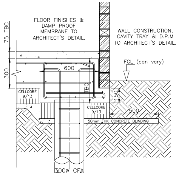
TYPICAL GARAGE SLAB DOWNSTAND DETAIL WITH HEAVE PRECAUTIONS
