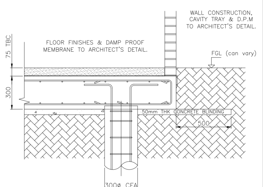
TYPICAL GARAGE SLAB EDGE DETAIL WITHOUT HEAVE PRECAUTIONS
