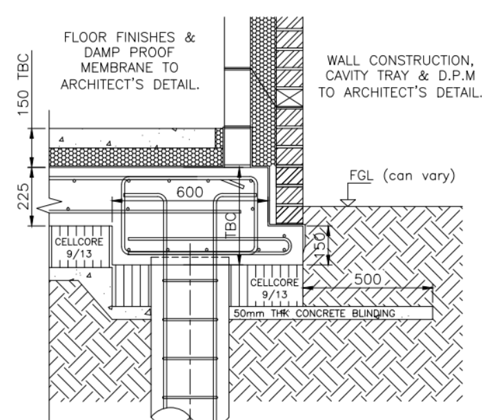
TYPICAL HOUSE SLAB DOWNSTAND DETAIL WITH HEAVE PRECAUTIONS
