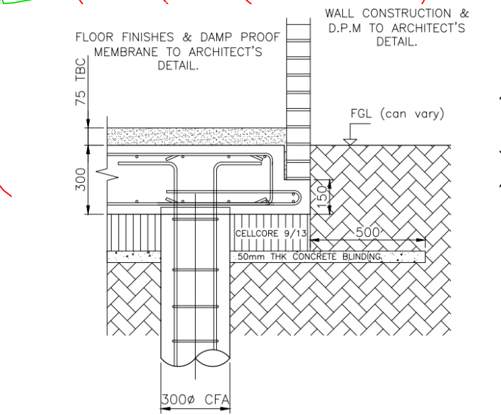
TYPICAL GARAGE SLAB EDGE NIB DETAIL WITH HEAVE PRECAUTIONS
