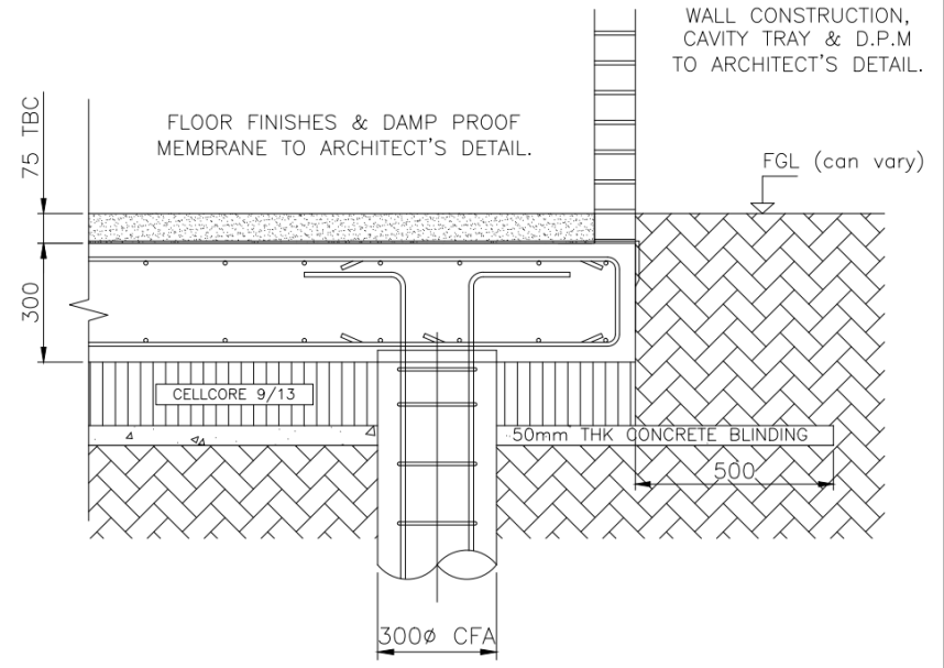
TYPICAL GARAGE SLAB EDGE DETAIL WITH HEAVE PRECAUTIONS
