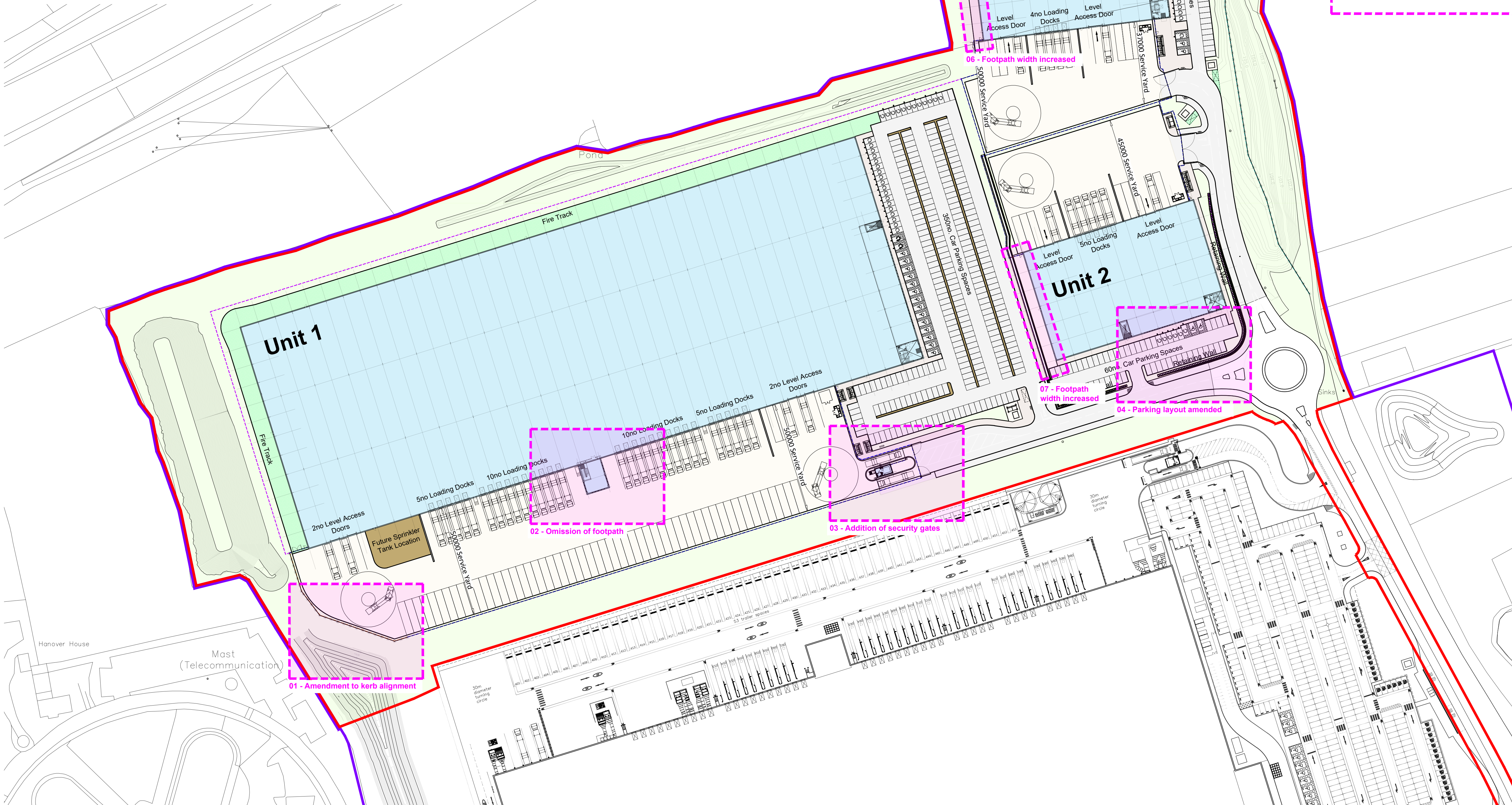
Site Masterplan Scale 1:1000 @ A0
