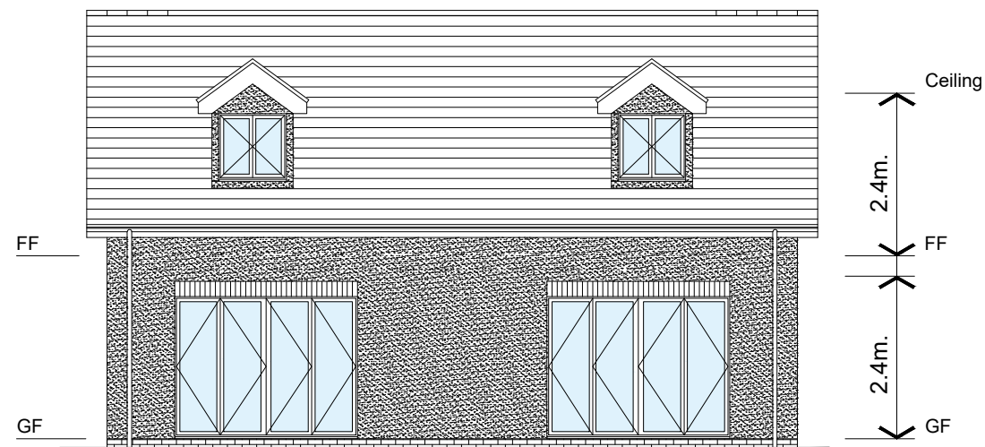
South elevation.
