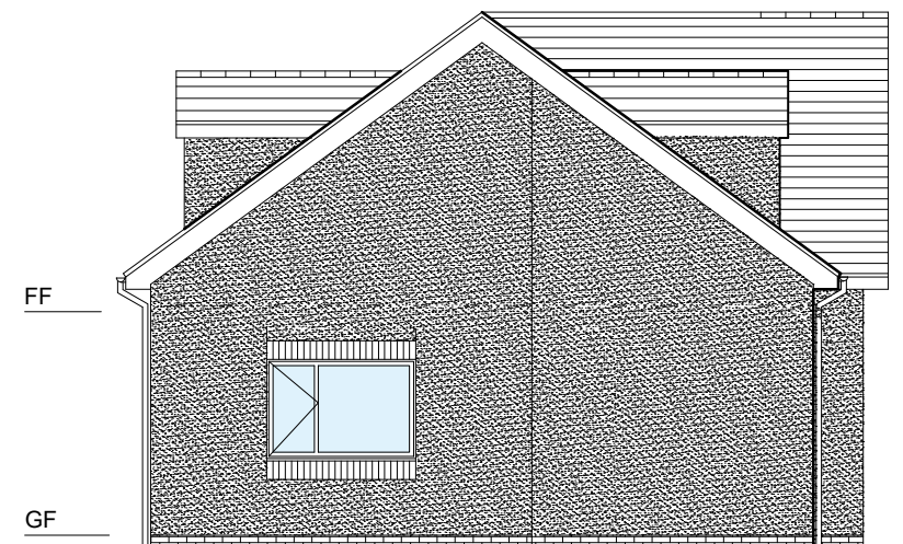
East elevation.
