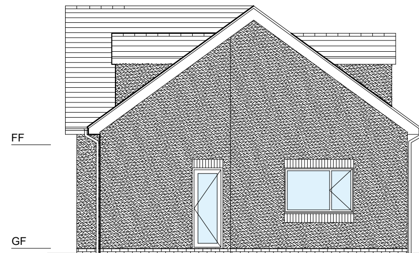
West elevation.
