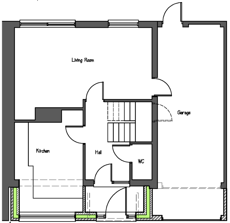
Proposed Plan 1:100
