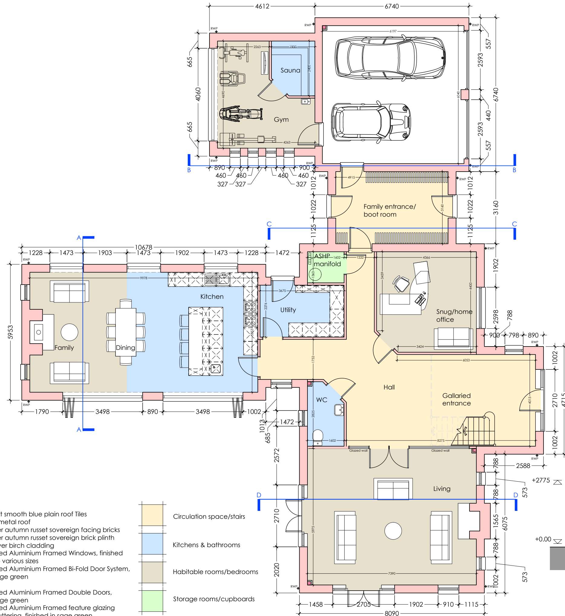
Ground floor plan 4 bed house 367.91m 2 (3,960.15sqft)
