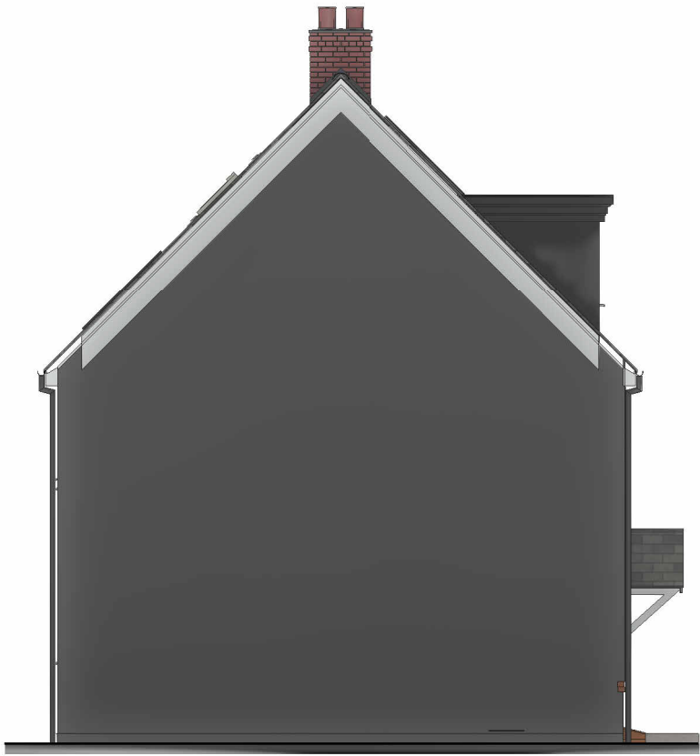
Side Elevation 1 : 100
