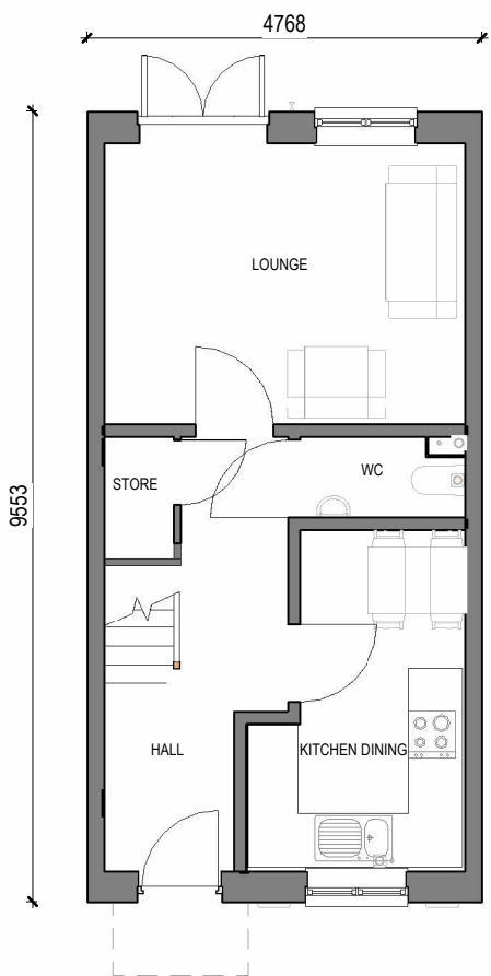
Ground Floor Planning
