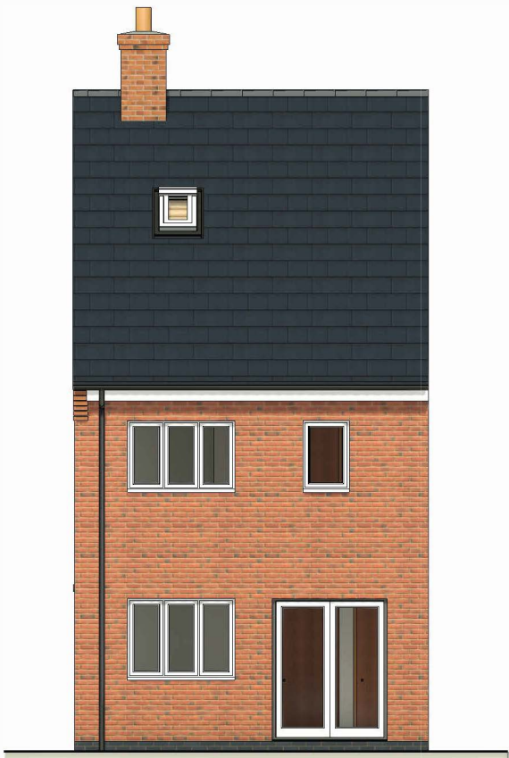
Rear Elevation 1 : 100
