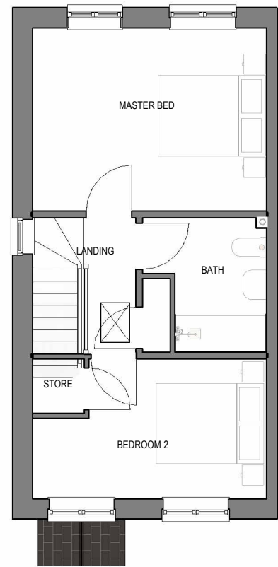
First Floor Planning
