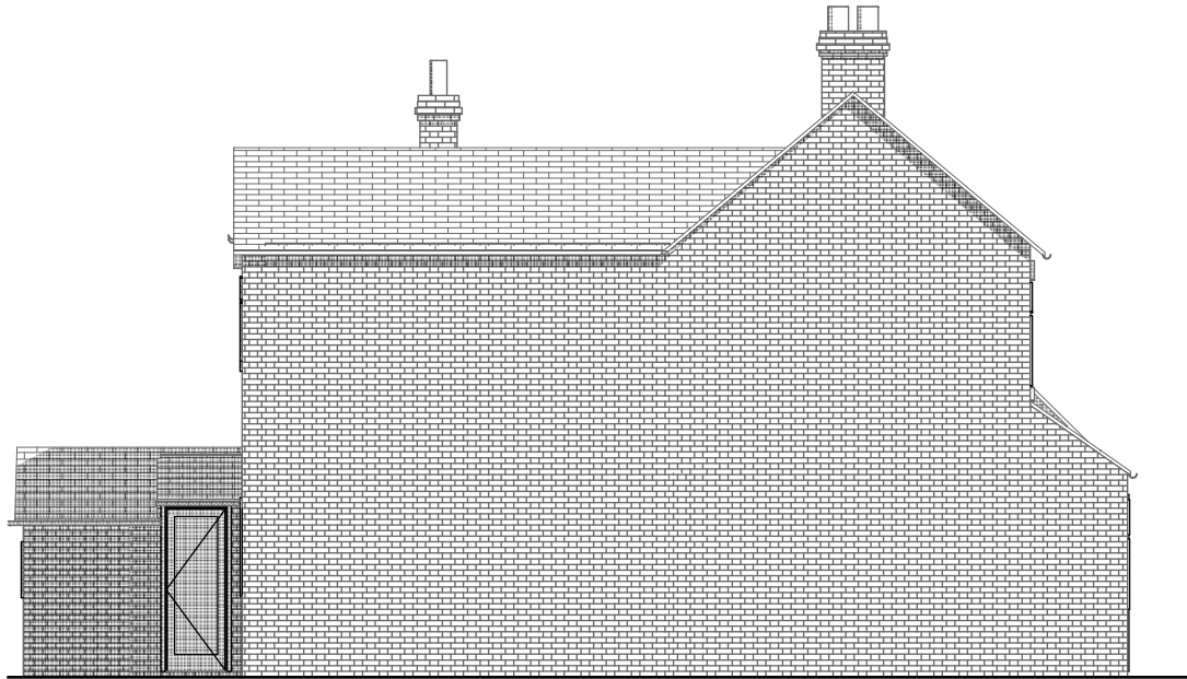
4 Side Elevation Two 1:100
