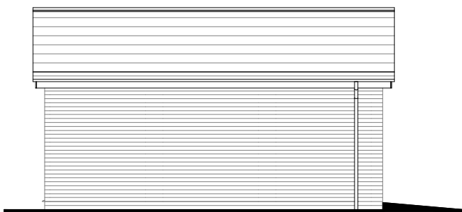
Side Elevation
