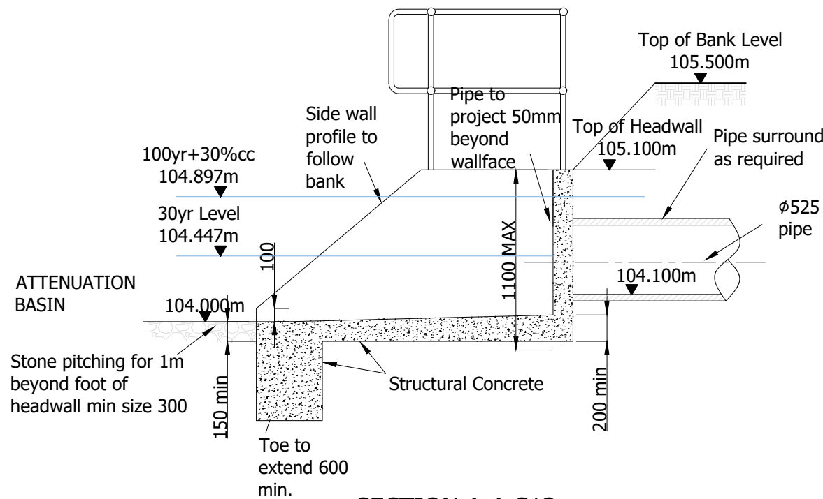
SECTION A-A S13
