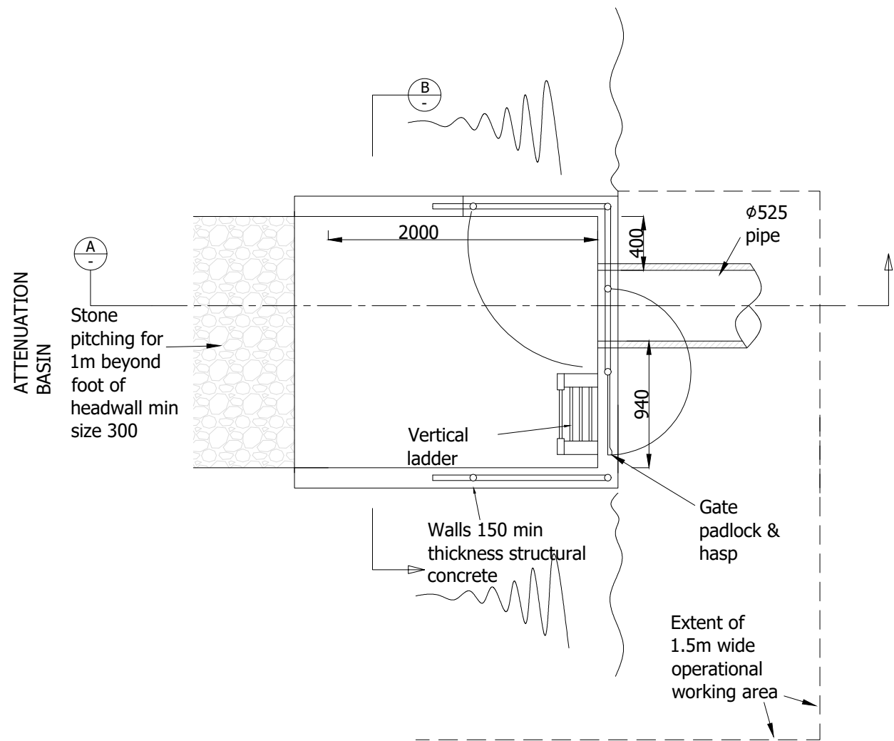
HEADWALLS 525mm DIAMETER PIPE PLAN REFER TO S13 ON DRAINAGE LAYOUT
