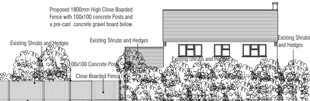
PROPOSED REAR (FENCING) ELEVATION
