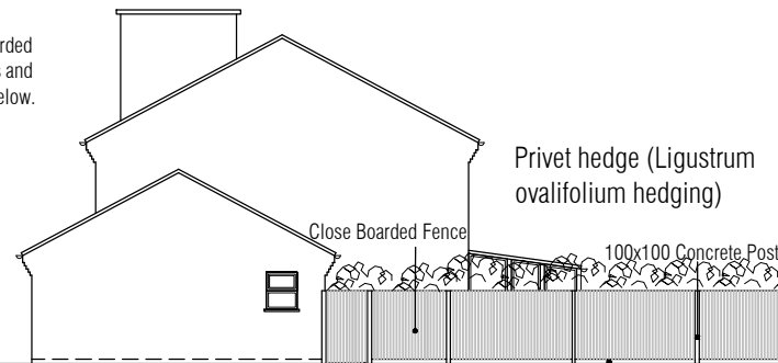
PROPOSED SIDE (FENCING)ELEVATION
