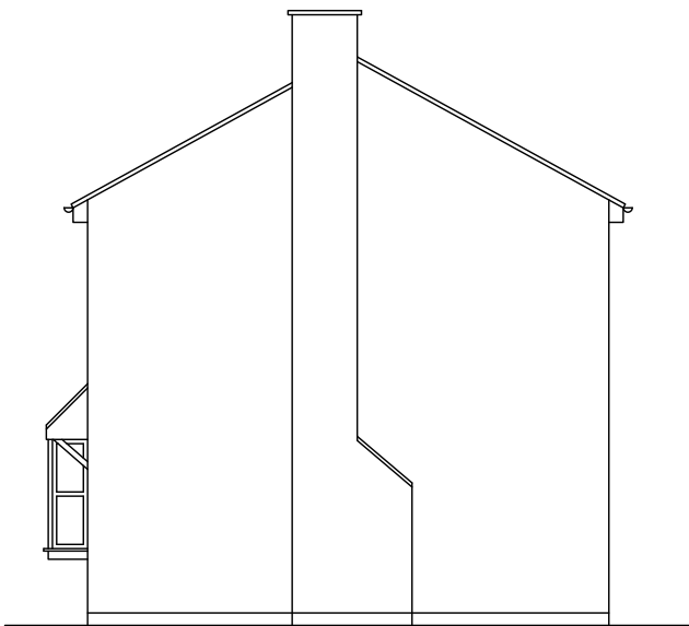
Side Elevation
