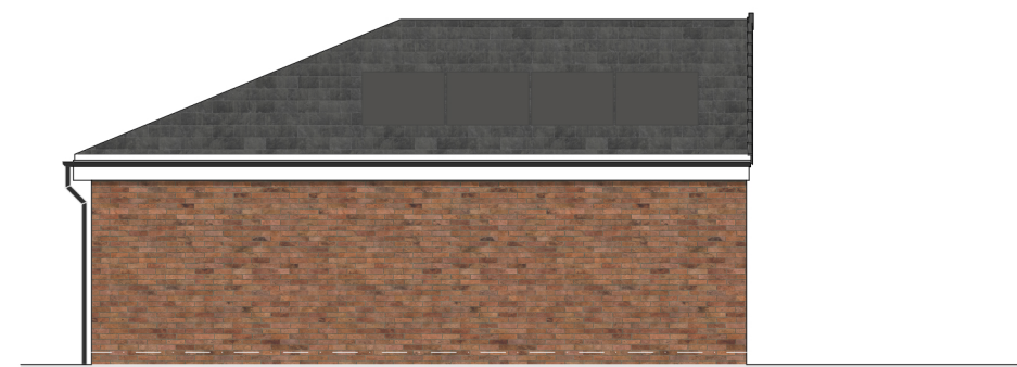
R.H. SIDE ELEVATION.
