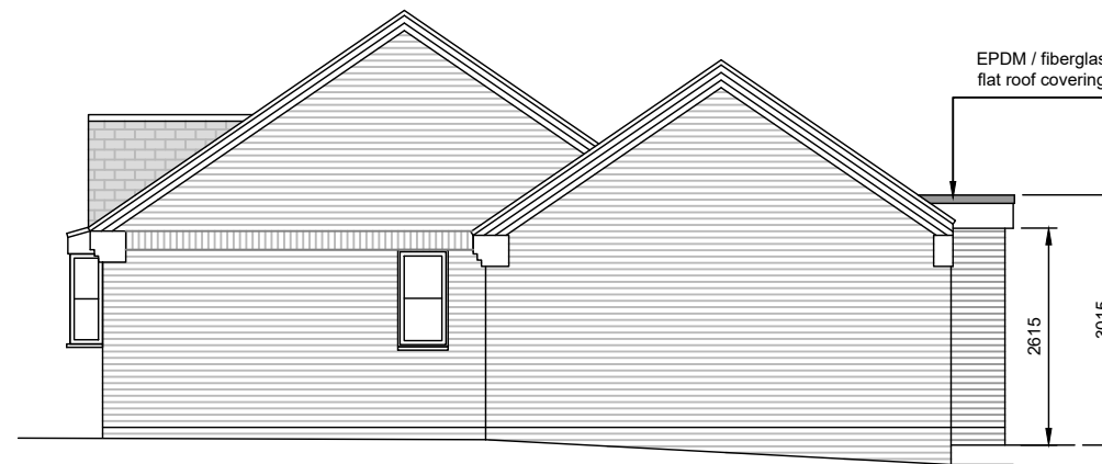
Proposed Right Elevation
