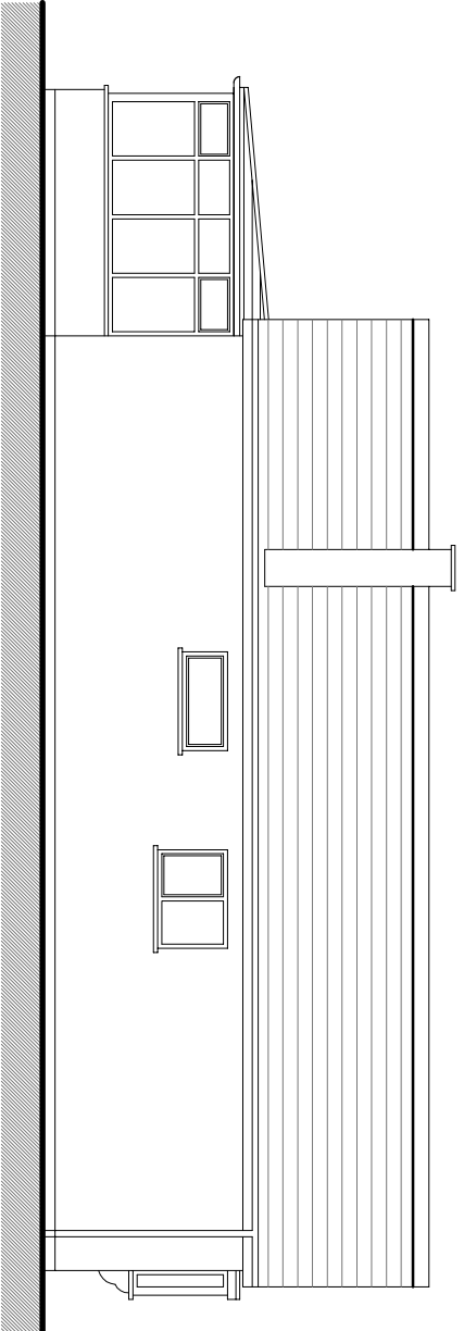
Existing Side Elevation (SW facing)
