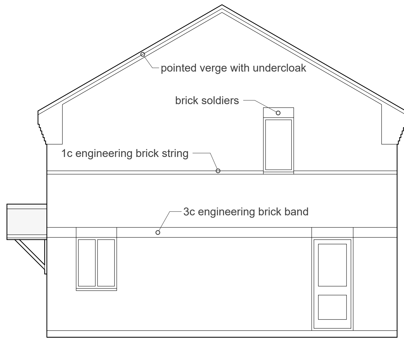
SOUTH ELEVATION
