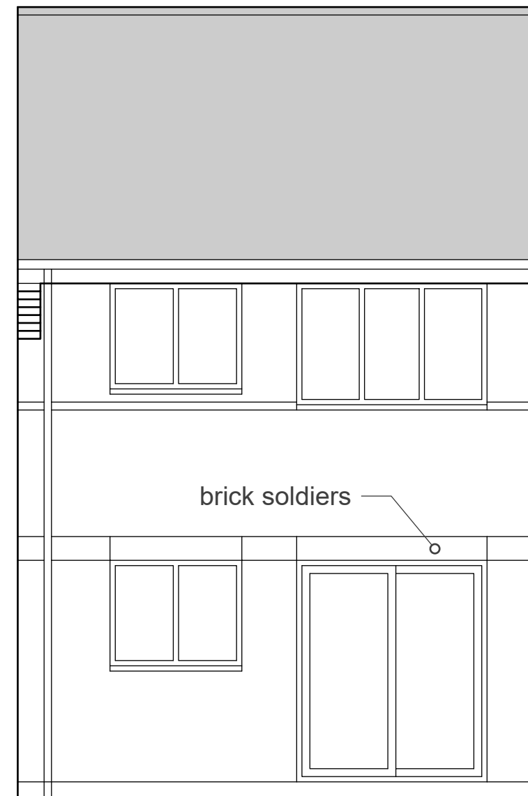
EAST ELEVATION
