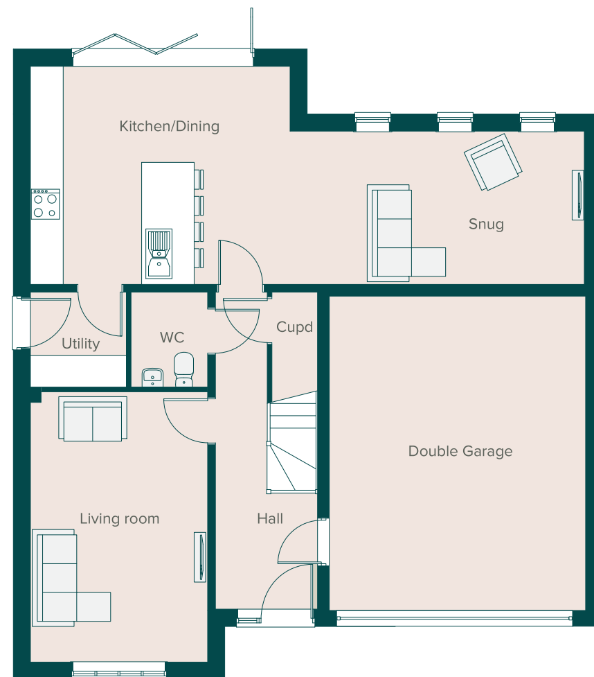
Ground Floor
