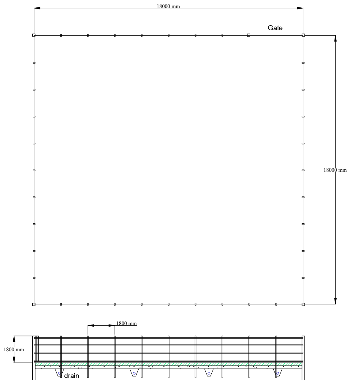
TYPICAL SECTION
