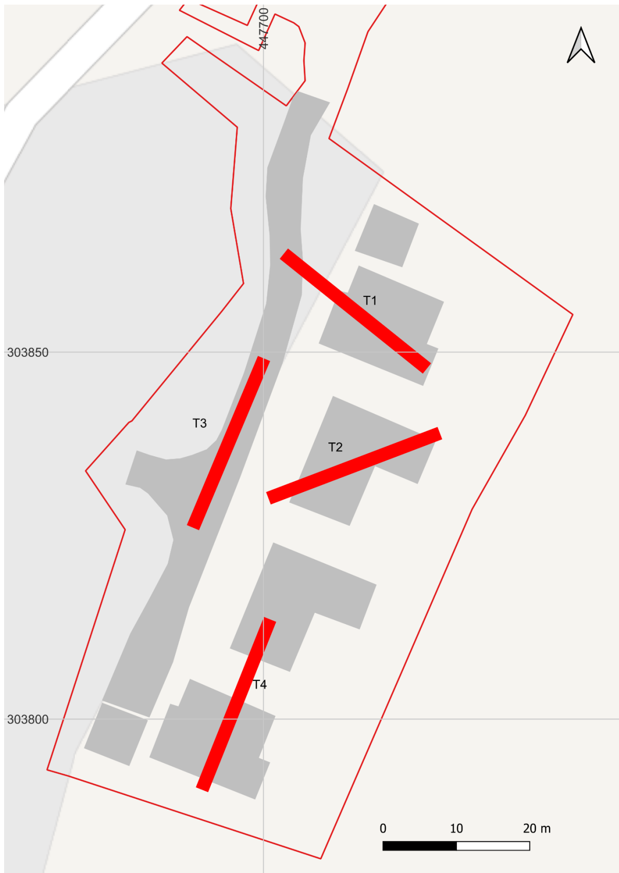
Figure 4: Proposed Trench plan overlain on proposed plans (grey shade).
