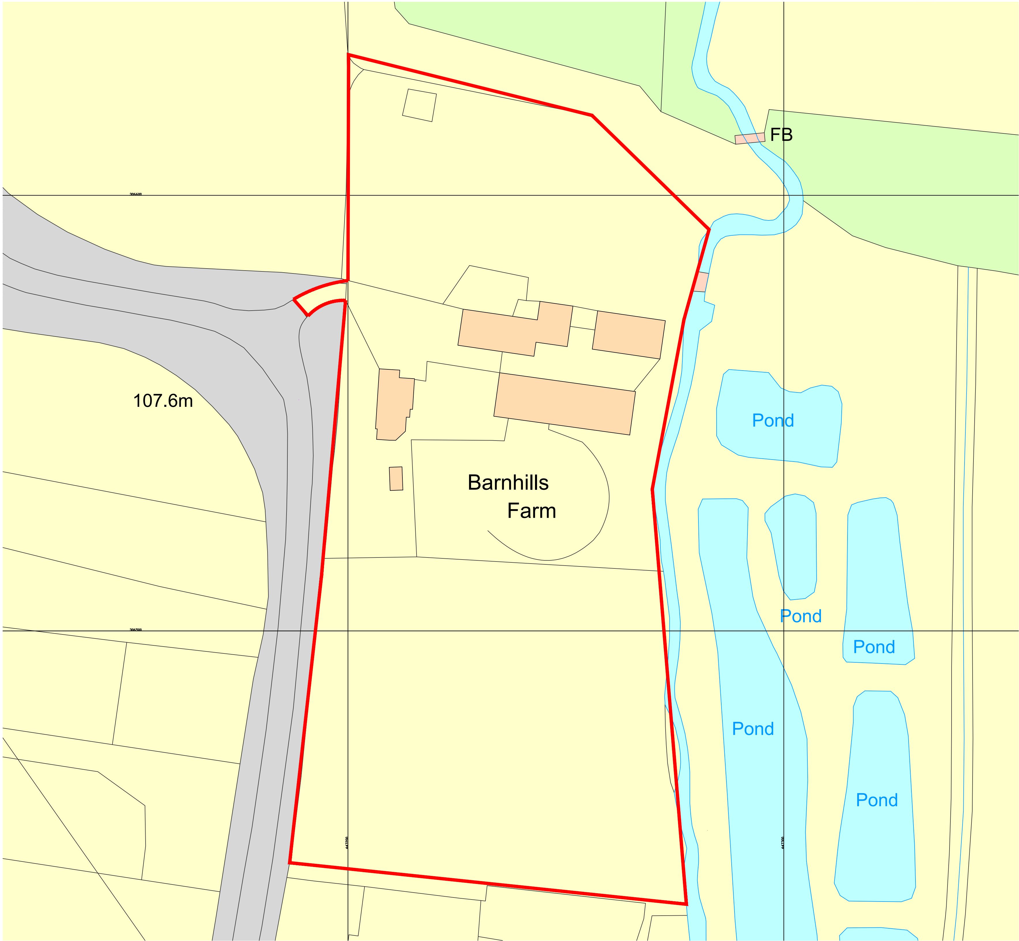
Location Plan 0 5m 10m 15m 20m 25m 1:500
