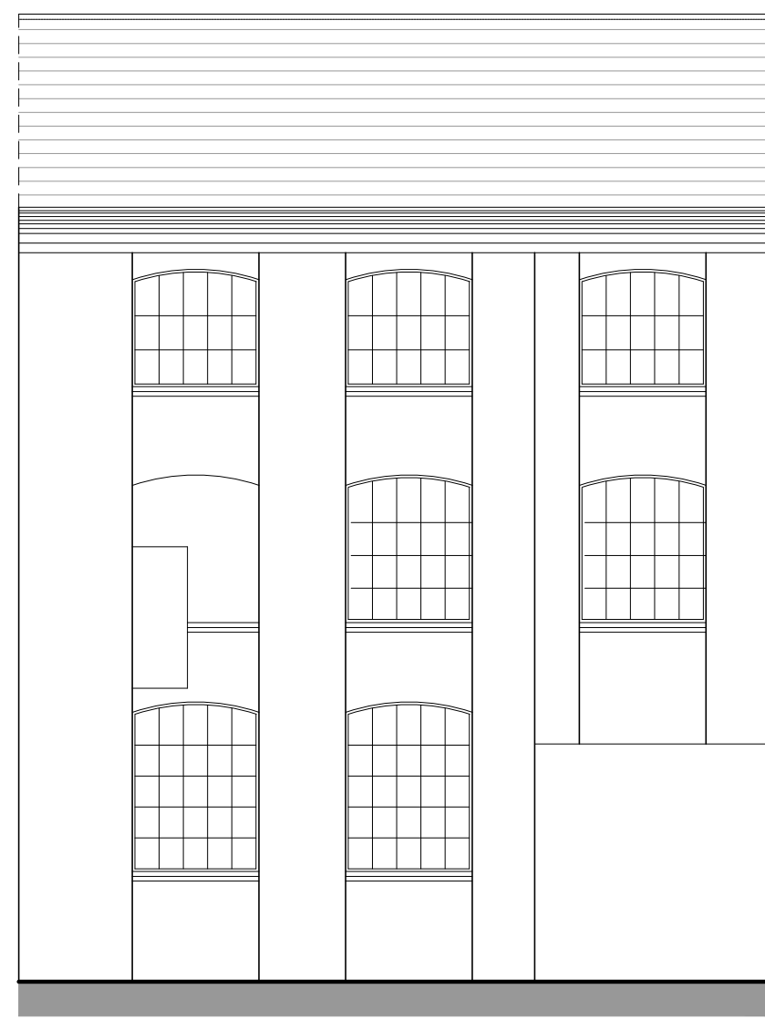
ELEVATION 01 (Courtyard Elevation Facing Upper Bond Street)
