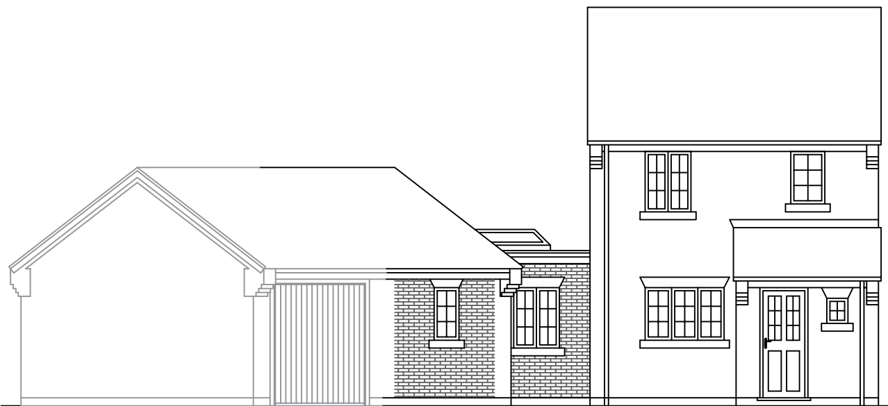
Proposed South East Elevation Scale 1/100
