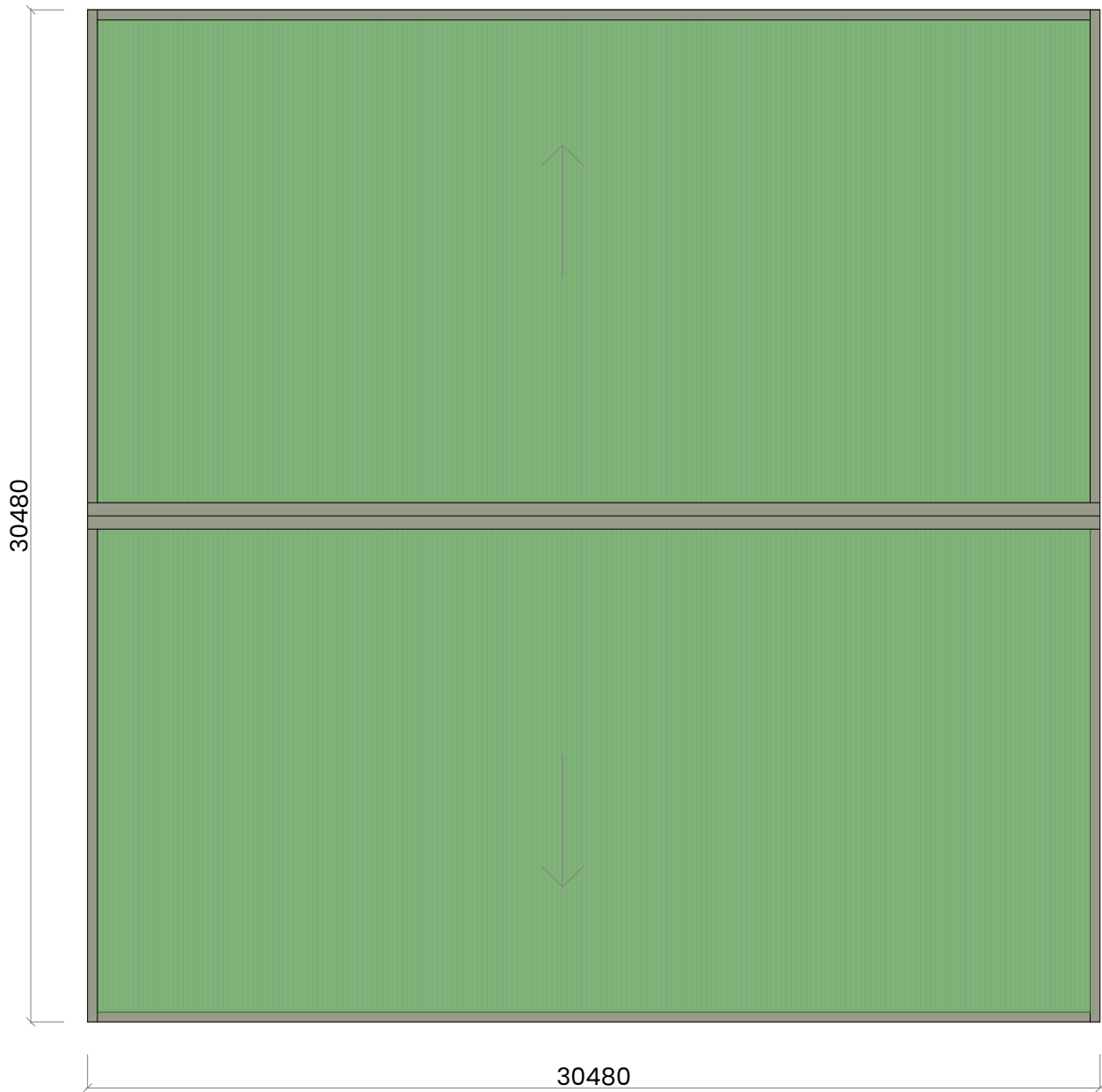
1:200 Roof Plan
