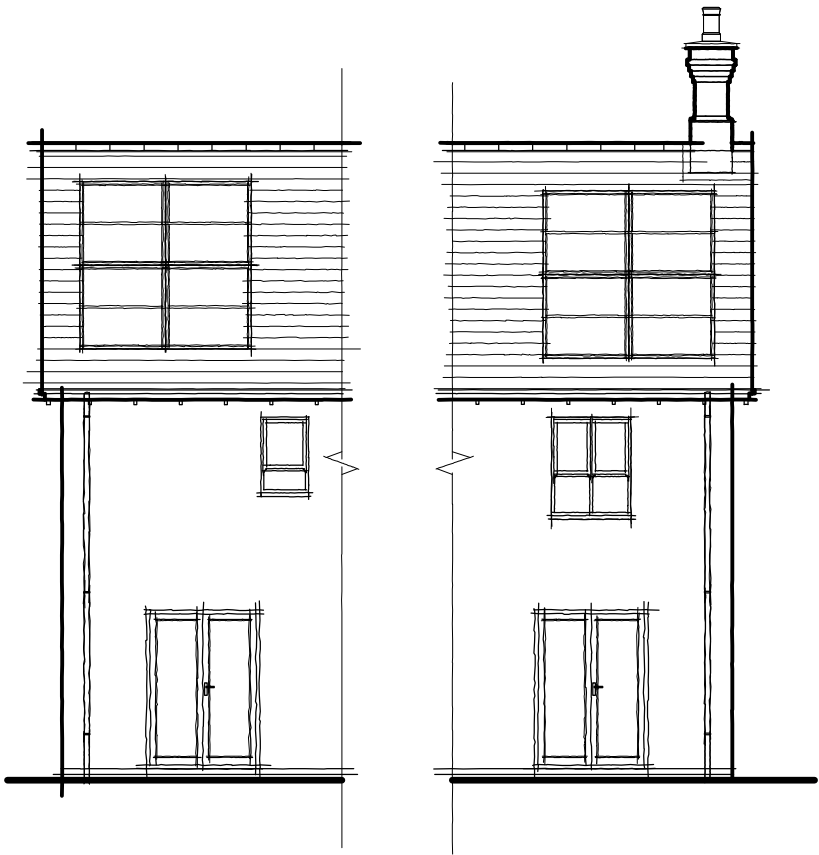
Rear Elevations
