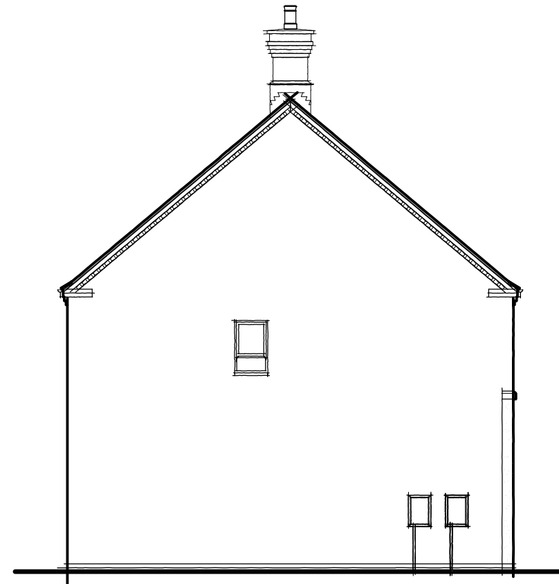
Side Elevation
