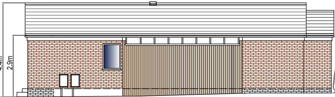
Proposed East Elevation Scale 1/100
