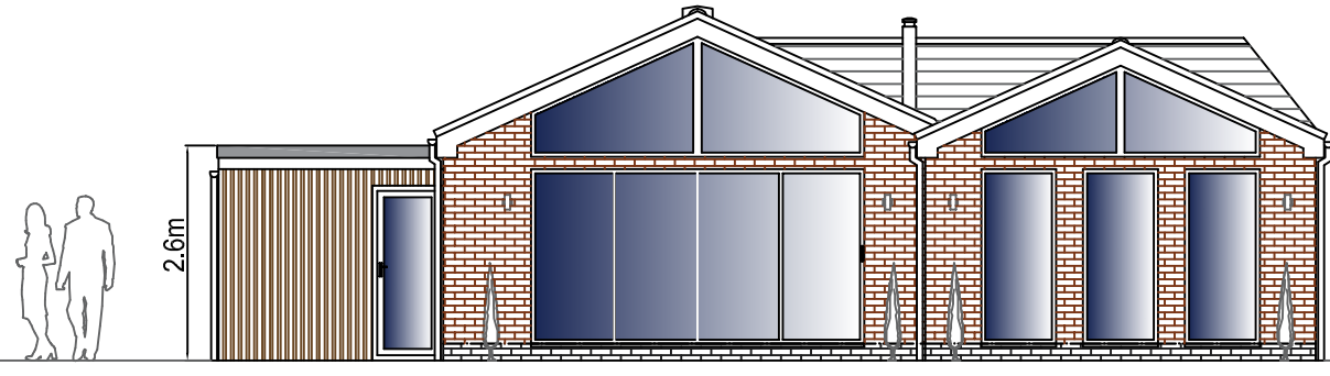
Proposed North Elevation Scale 1/100
