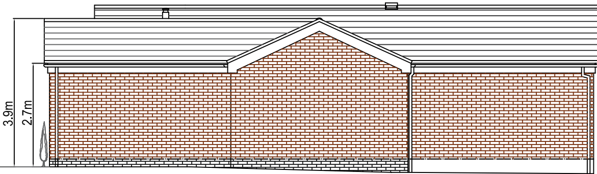
Proposed West Elevation Scale 1/100
