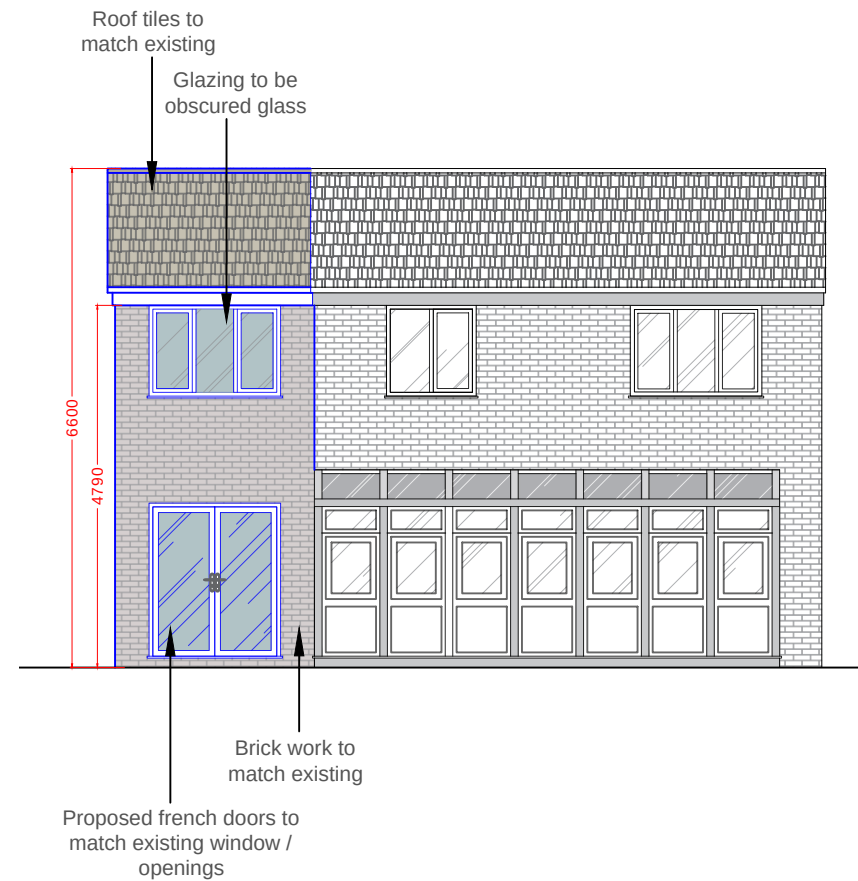
PROPOSED REAR ELEVATION 1:100 AT A3
